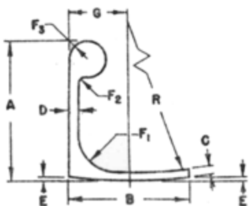
BAC 1515 BULB ANGLE MISCELLANEOUS
