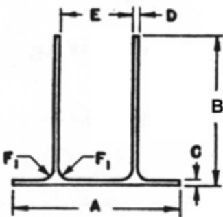
BAC 1507 TT SECTION EXTRUDED
